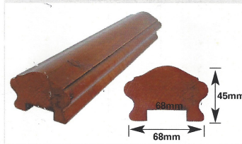
Superior Handrail
