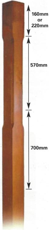
Stop Chamfered
